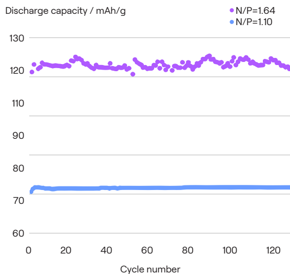
FIGURE 3: Cycling performance of LNMO–graphite cells with improved anode control
