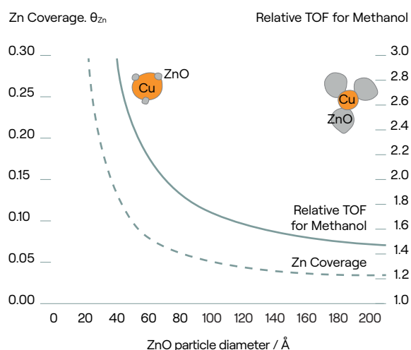
FIGURE 6: Zn coverage and methanol activity versus ZnO particle size
