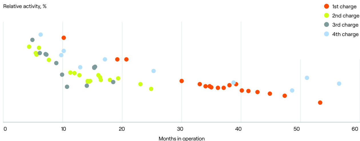
FIGURE 16: Activity trends of different MK-catalyst charges in CO 2 -rich gas
