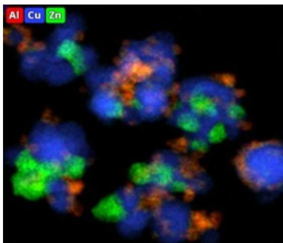
FIGURE 3: Imagery of a spent methanol catalyst
