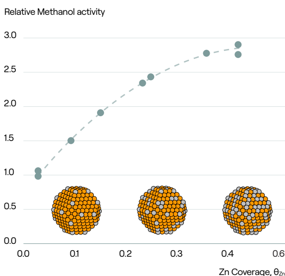
FIGURE 5: Methanol synthesis activity versus the fraction of Zn in the surface of the Cu particles
