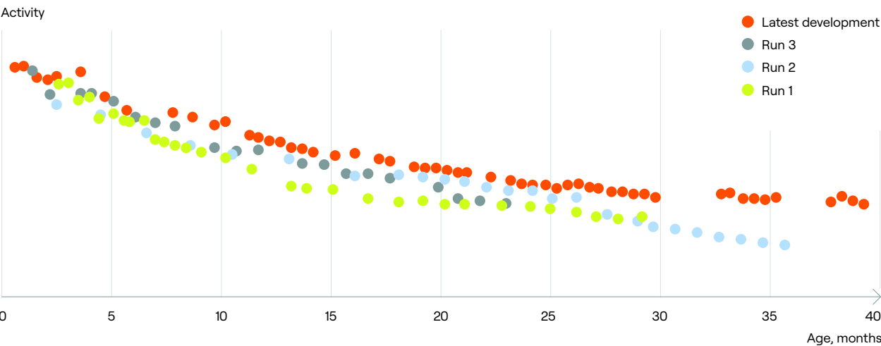
FIGURE 12: Comparison of activities for different charges of MK catalysts
