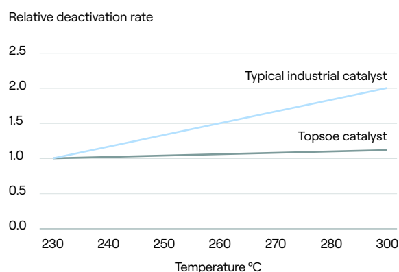
FIGURE 8: Relative deactivation rates of a typical industrial methanol catalyst and a Topsoe methanol catalyst, plotted vs. temperature
