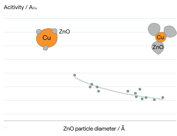
FIGURE 7: Activity divided by Cu surface area, plotted as a function of ZnO particle size
