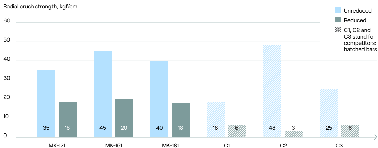
FIGURE 11: Mechanical strength of methanol catalysts in oxidized and activated states
