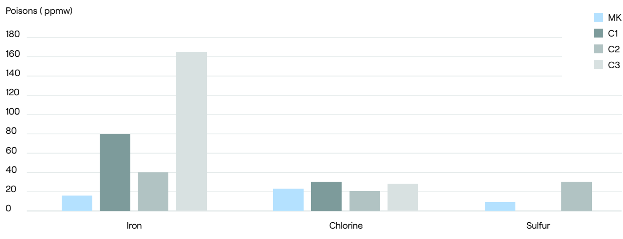
FIGURE 10: Figure 10: Impurity levels in four different catalysts
