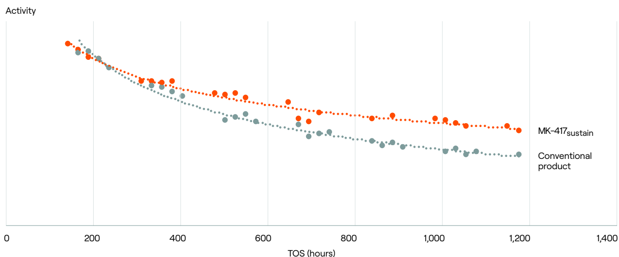
FIGURE 15: Activity levels of a classical Topsoe product and MK-417 SUSTAIN™ in a synthesis gas with a high CO 2 partial pressure (>10 bar)
