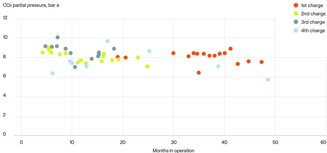
FIGURE 17: CO 2 partial pressure for different MK-catalyst charges in CO 2 -rich gas
