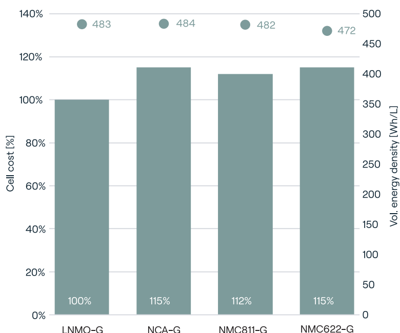
Figure 7: Comparison of cell cost per kWh for large format cells in 4 kWh battery module with LNMO, NCA and NMC cathodes and graphite anode. Cell calculations are performed using BatPac 3.0.
