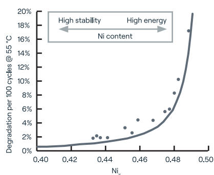
Figure 6: a: Correspondence between the Ni-content in LNMO, b: particle size and c: morphology and the degradation per 100 cycles measured for LNMO–lithium cells at 55 °C. To obtain a low degradation, the spinel should have a low Ni content, a small diameter and a spherical shape.
