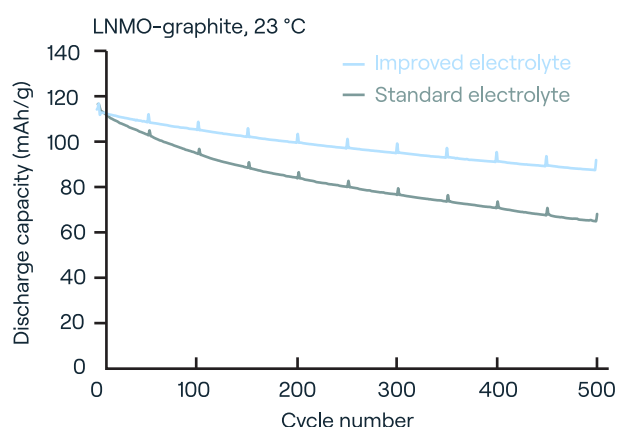
Figure 3: Cycling curves of LNMO-graphite cells at 1C discharge and 0.5C charge with TBM-129 cathode at a: 23 °C and b: 45 °C with two stages of system optimization.
