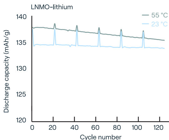
Figure 2: Cycling curves at 1C of TBM-129 in LNMO-lithium cells at room temperature and 55 °C. Every 20 th cycle is performed at 0.2C. b: Voltage curve of LNMO-lithium during charge and discharge.
