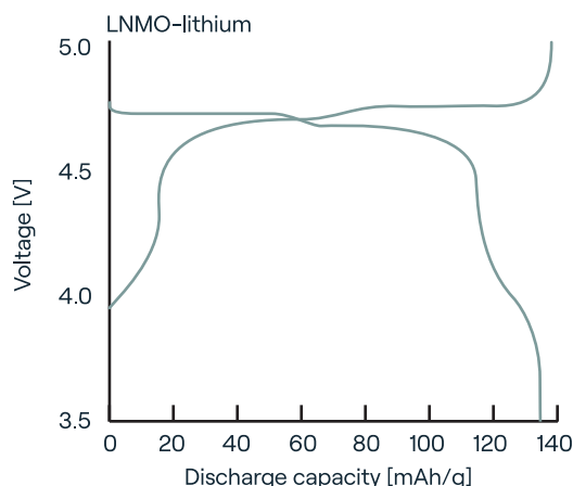
Figure 2: Cycling curves at 1C of TBM-129 in LNMO-lithium cells at room temperature and 55 °C. Every 20 th cycle is performed at 0.2C. b: Voltage curve of LNMO-lithium during charge and discharge.
