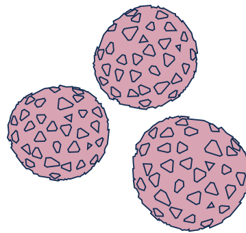
Figure 5: Different strategies pursued at Haldor Topsoe to improve performance of the LNMO material. In addition to TBM-129 (a), Topsoe is developing a single-crystal LNMO material (b) and LNMO materials with coating and doping (c).
