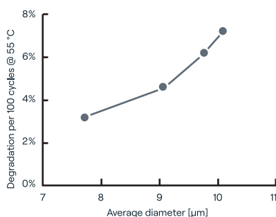
Figure 6: a: Correspondence between the Ni-content in LNMO, b: particle size and c: morphology and the degradation per 100 cycles measured for LNMO–lithium cells at 55 °C. To obtain a low degradation, the spinel should have a low Ni content, a small diameter and a spherical shape.
